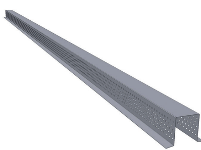
KALDHARJA TUGILIIST RR 23, 40 x 40 x 40 mm, L=2 000 mm
